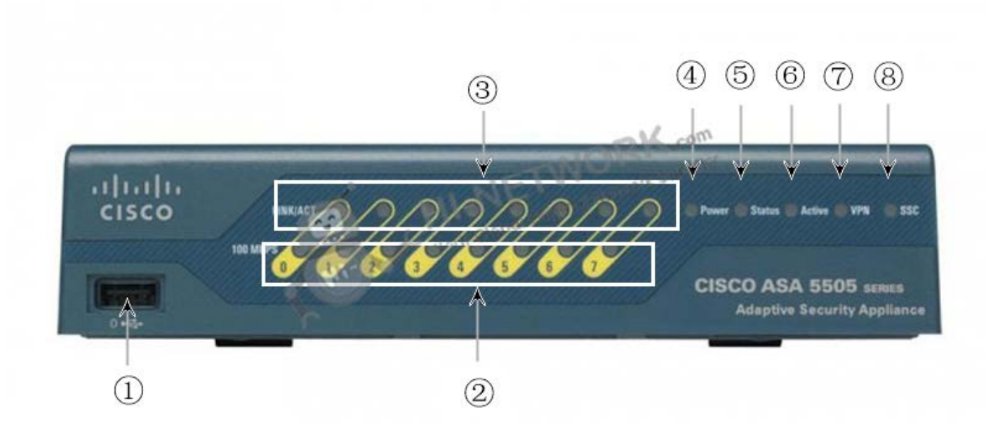
Figure 2 shows the front view of ASA5505-K8.
